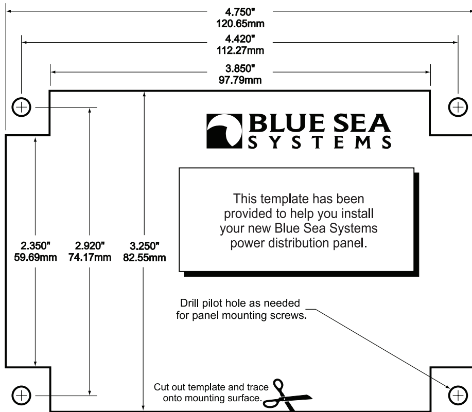
Panel Template AC Source Selector Panel PN 8365 / PN 8367
