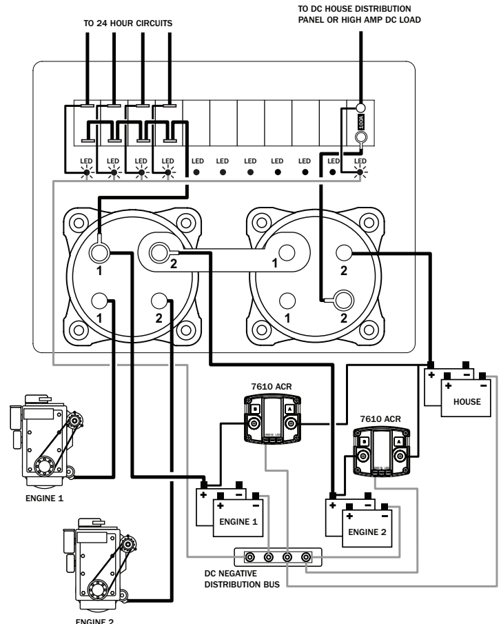
Wiring Diagram 8693
