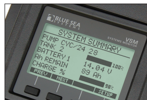
VSM 422 monitors four vessel systems AC, DC, tank, and bilge
